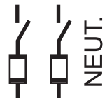
Fusible, Two-pole, 120/240 and 240 Volts ac; 250 Volts dc (30-100 amps only); Three-wire SN, 240 Volts ac
