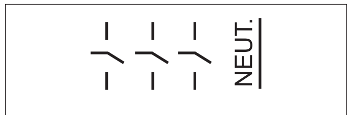
Four-wire SN, 240 Volts ac, No Fuse
