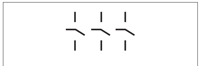
Three-pole, 240 Volts ac, 250 Volts dc, No Fuse
